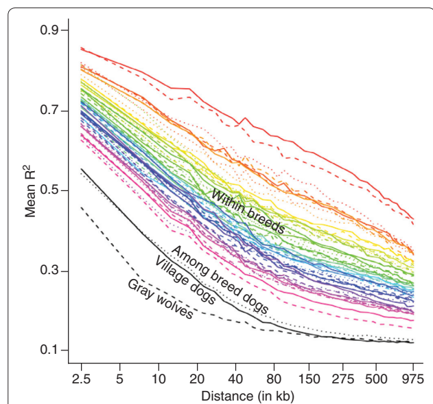
Figure 3. Decay of linkage disequilibrium (LD) among dogs and gray wolves. Among dog breeds (black dotted line); among gray wolves (dashed black line); within a population of village dogs (solid black line); and within dog breeds (colored lines). R^2 is square of the coefficient of association of allele frequencies between two loci [76]. Between breeds and within village dogs, LD extends for approximately 100 kb (roughly the equivalent of LD in humans). LD tracks are somewhat shorter in wolves and at least ten-fold longer within breeds (adapted from [8]).
